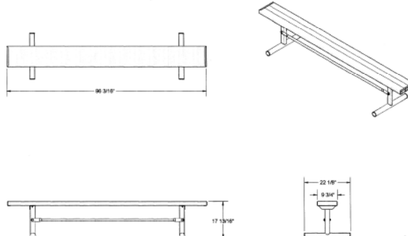
8' Park Bench, No Back - 2" x 10" Aluminum Plank
