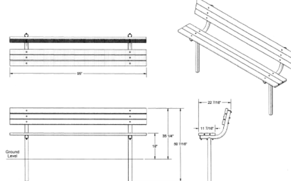
8' Park Bench with Back - 2" x 4" Planks
