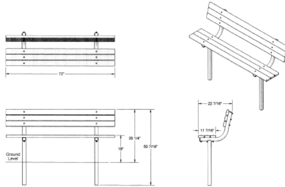
6' Park Bench with Back - 2" x 4" Planks
