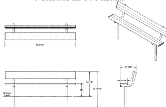
8' Park Bench with Back - 2" x 10" Seat & Back
