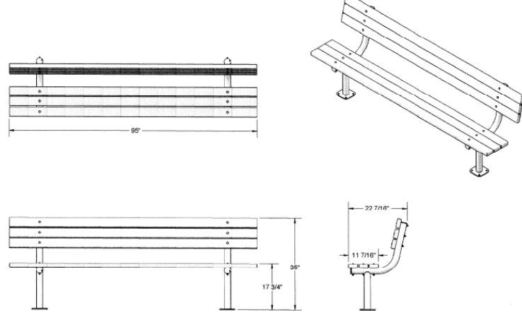
8' Park Bench with Back. 2" x 4" Wood Planks
